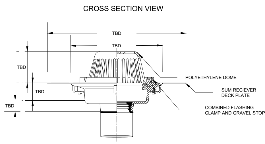
OVERFLOW STRUCTURE - DEBRIS CAGE
